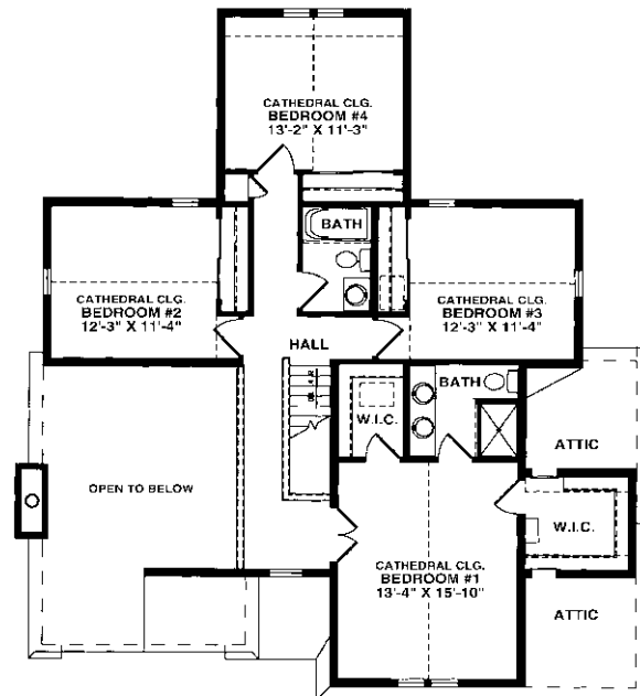
2nd Floor - 1,213 square feet of living area
